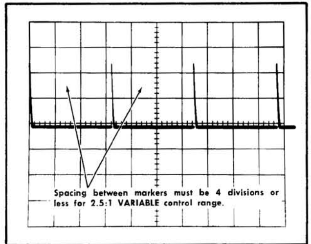
Fig. 5-16. Typical CRT display showing adequate VARIABLE TIME/DIV control range.
